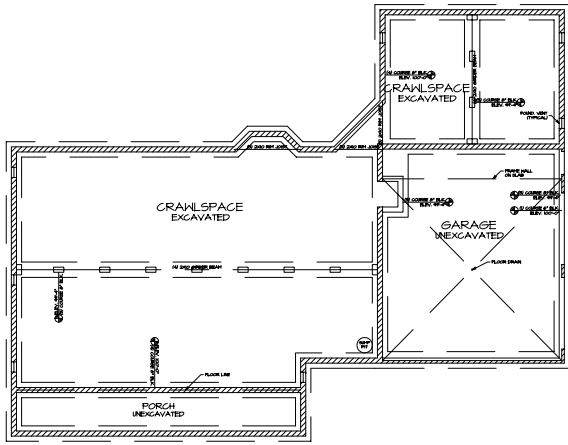
1-1 FOUNDATION PLAN A-2 SCALE: 1/4"=1'-0"
