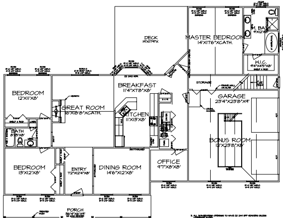
1-1 FIRST FLOOR PLAN A-3 SCALE: 1/4"=1'-0"
